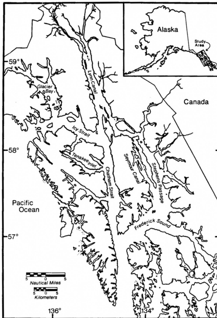
Figure 1. The southeastern Alaska study area.
